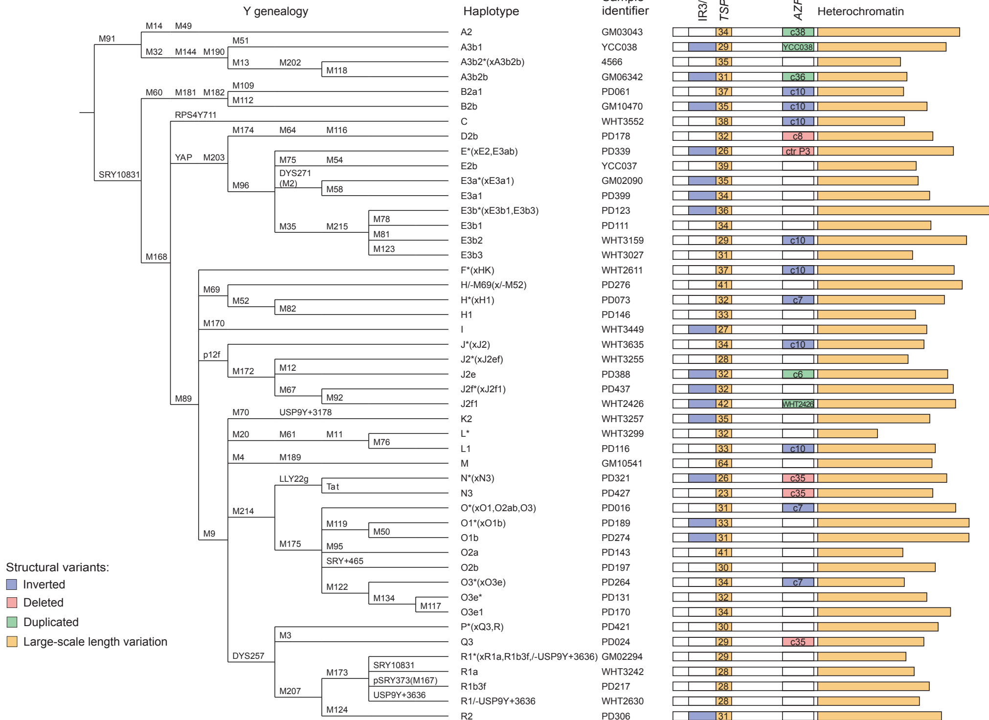
Repping et al. Supplementary Figure 1 Y-chromosome genealogical tree and structural polymorphisms identified, with sample identifiers and haplotype designations.
