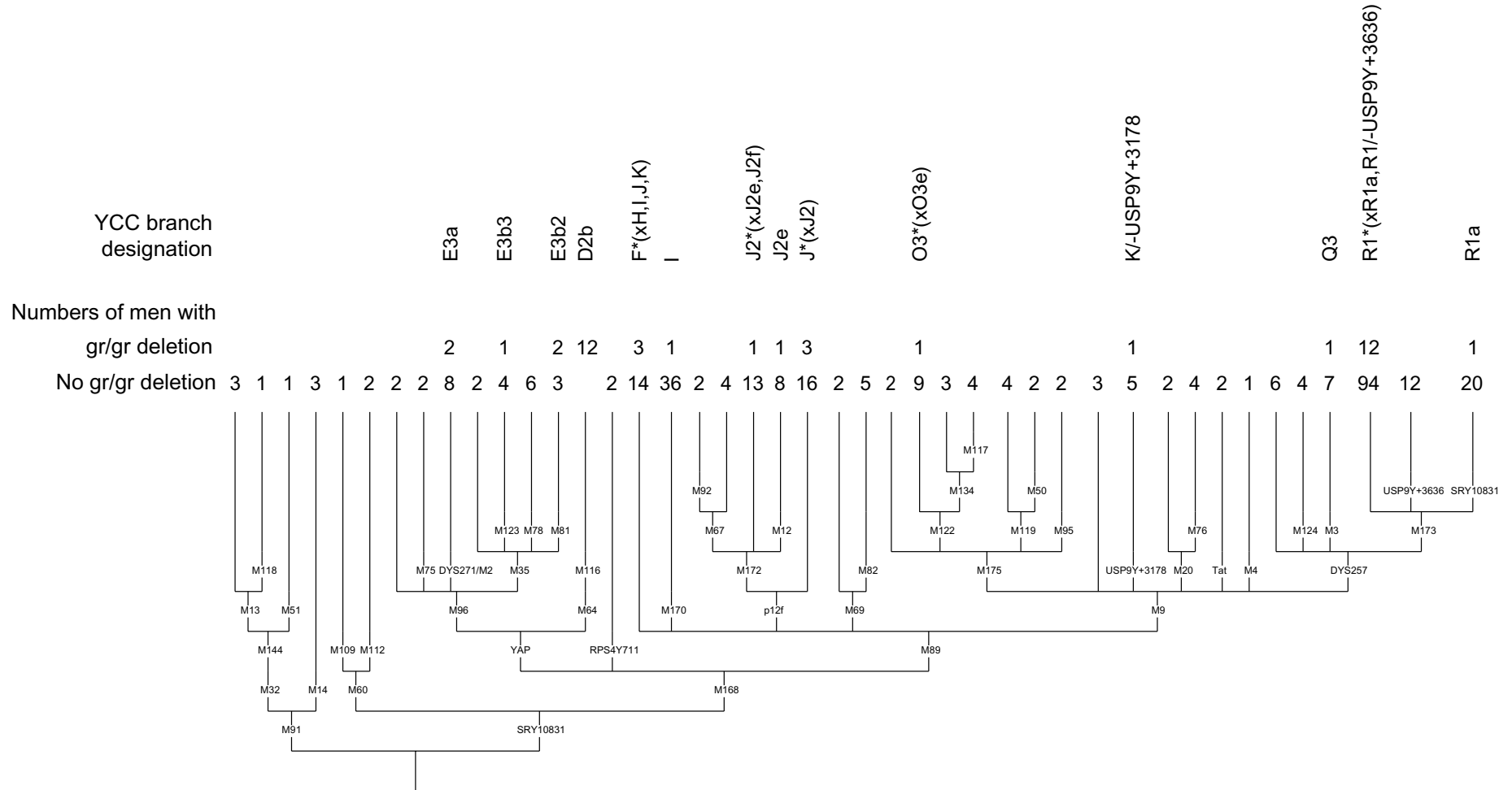
Supplementary Fig. 1 Y genealogy from Fig. 4 (main text) with Y Chromosome Consortium (YCC) branch designations ( Genome Res. 12 , 339-348, 2002)
