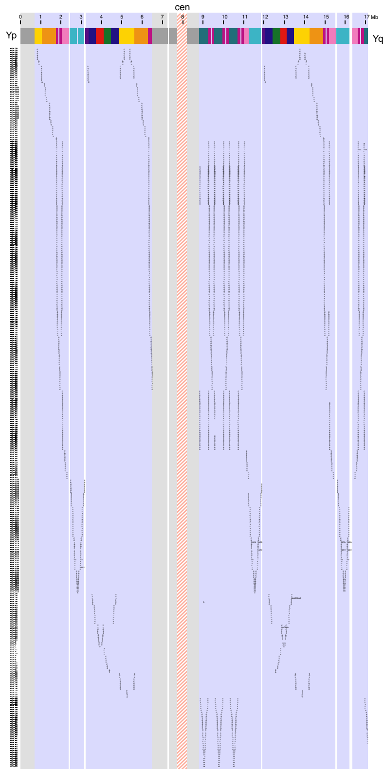
Supplementary Figure 2 Positions of informative sequence family variants (SFVs) along chimpanzee ampliconic sequence. Each row represents one SFV. Numbers at left refer to PCR assay. The letters in each row represent sequence content of the SFVs within amplicon copies. There are multiple SFVs for each PCR assay in almost all cases. SFVs from P6, P7, and P8, which are embedded in X-degenerate sequence, are not shown. Sequences of PCR primers and amplification products are given in supplementary file 1.
