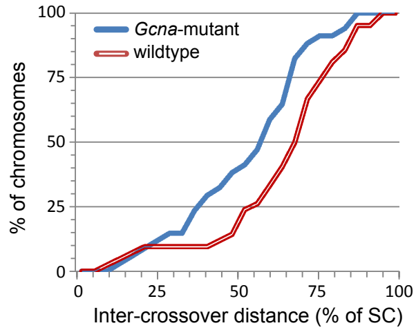
Figure S6: Related to Figure 6. Cumulative distribution curves of the distance between two MLH1 foci in wild-type and mutant bivalents (Chromosomes 11-13). Crossover interference gamma shape parameter for wild type is 11.037 and mutant is 9.479 (Two-sided Mann-Whitney; p=0.0074 ).
